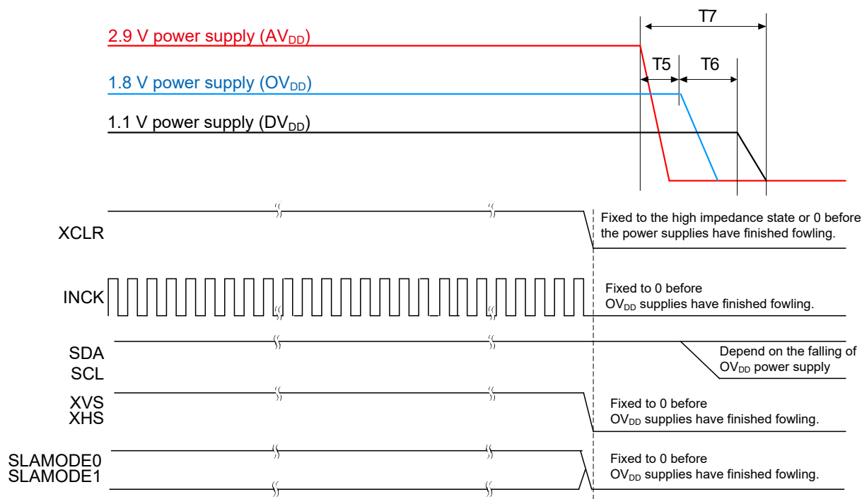
Power-off Sequence
