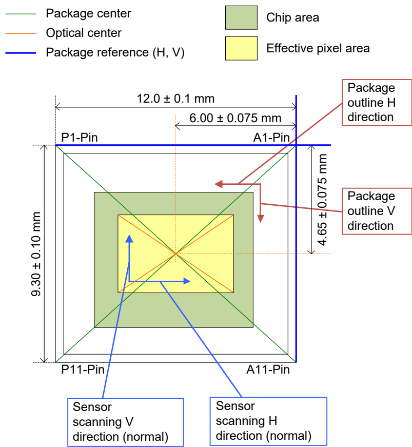
Optical Center
